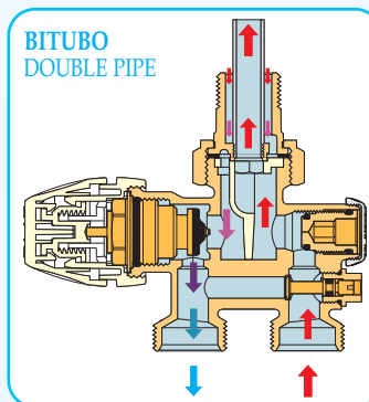
Collegamento standard Standard connection
