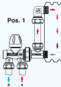
Collegamento standard Standard connection
