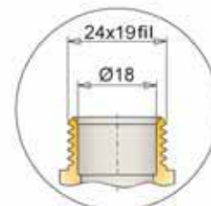
Art. 1666K per tubi multistrato for multilayer pipe Ø16x2,0 Ø18x2,0 Ø20x2,0
