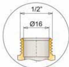
Art. 1668 (1/2") per tubi multistrato for multilayer pipe Ø14x2,0 Ø16x2,0 Ø18x2,0 Ø20x2,0
