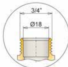
Art. 1666 per tubi multistrato for multilayer pipe Ø14x2,0 Ø16x2,0 Ø18x2,0 Ø20x2,0
