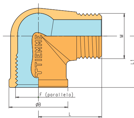
ART. 1561 raccordo curvo maschio/femmina ART. 1561 elbow male/female connector
